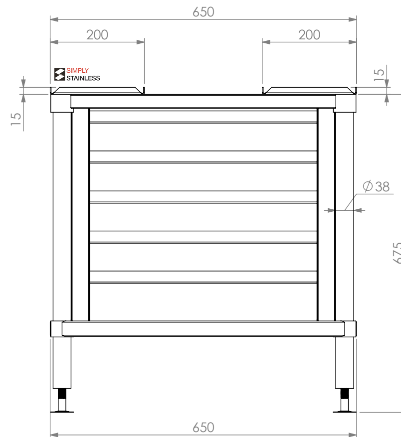
SIDE ELEVATION
